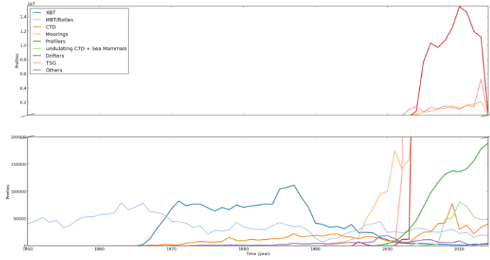
Figure 1: Yearly number of distributed profiles, sorted by instrument types.
