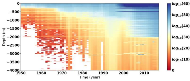
Figure 2: Yearly number of measurements as a function of depth.
