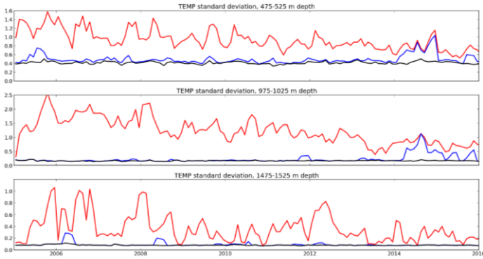
Figure 10: Mean temperature standard deviation in the 475-525 m depth layer (top), 975-1025 m depth layer (mid.) and 1475-1525 m depth layer (bot.) The raw dataset (red), NRT dataset (blue) CORA dataset (black) are represented.
