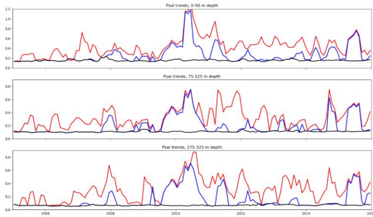
570 Figure 7: Mean salinity standard deviation in the 0-50m layer (top), 75-125 m depth layer (mid.) and 275-325 m depth layer (bot.). The raw dataset (red), NRT dataset (blue) CORA dataset (black) are represented.
