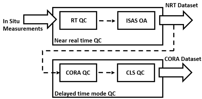
560 Figure 4: Coriolis database validation process.
