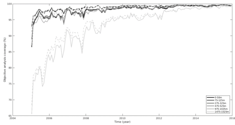
Figure 5: Coverage of the Temperature and Salinity objective analysis for temperature (dashed line) and salinity (hard line) objective analysis.
