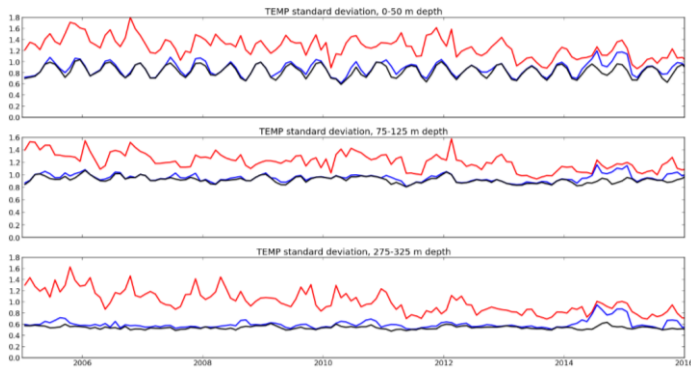
Figure 9: Mean temperature standard deviation in the 0-50m layer (top), 75-125 m depth layer (mid.) and 275-325 m depth layer (bot.). The raw dataset (red), NRT dataset (blue) CORA dataset (black) are represented.
