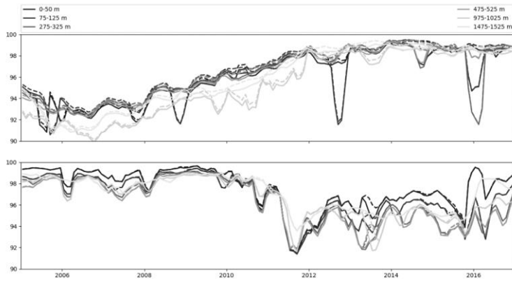
Figure 6: Percentage of good flags (flags 1 and 2) in the analyzed layers for the NRT dataset (hard line) and for the CORA dataset (dashed line). Upper panel for temperature, lower panel for salinity
