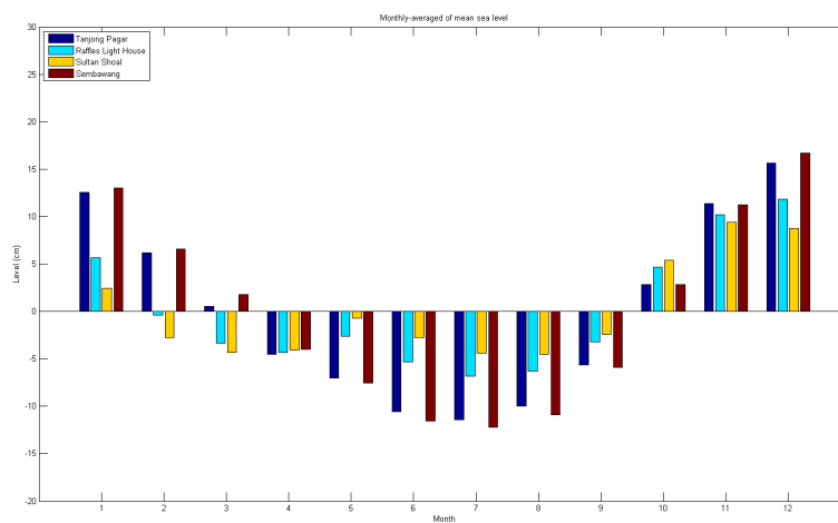
Fig. 3. Monsoonal and seasonal influence on sea level variations (monthly sea level).
