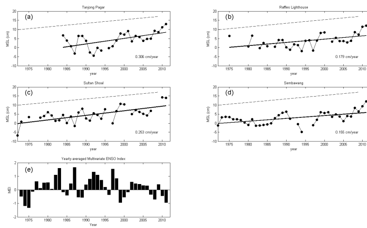
Fig. 4. Trends of annual MSL at (a) TP, (b) RL, (c) SH and (d) SE, in correspondence with (e) ENSO index. Thick lines represent tendency from local MSL; dash lines indicate global trend during 1972–2009.
