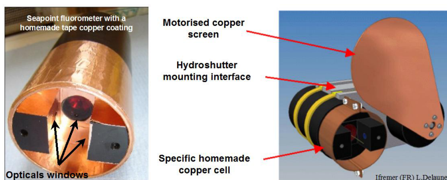
Fig. 4. Biofouling protection with a motorized copper shutter.
