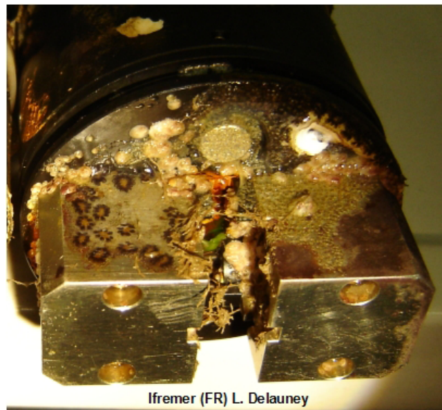
Fig. 1. Fluorometer after 30 days in Helgoland (Germany) during summer.
