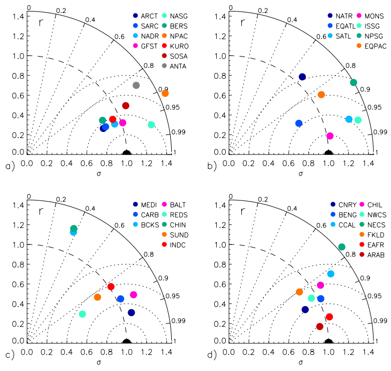
Fig. 10. Same as Fig. 9 for the pair SeaWiFS/MERIS.
