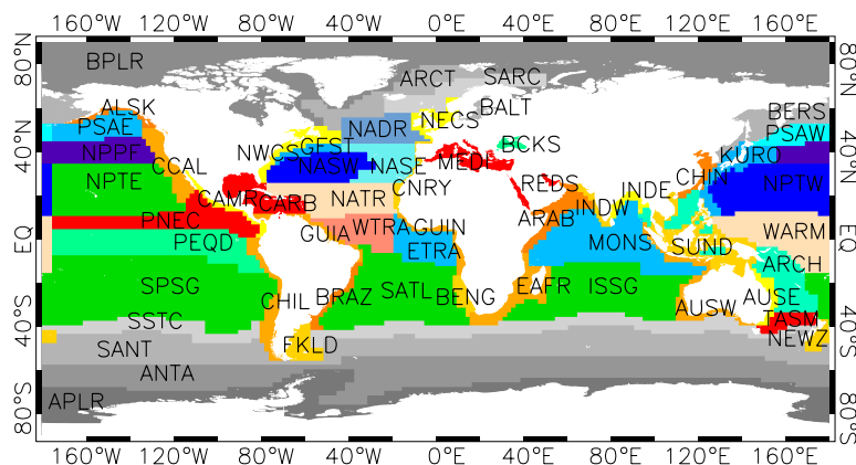
Fig. 1. Definition of the provinces used for statistical analyses.
