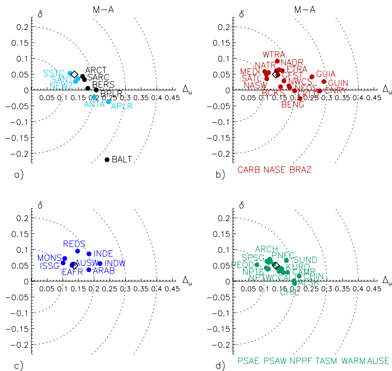
Fig. 8. Same as Fig. 6, for the pair M–A (MERIS versus MODIS Aqua), for the period 2003–2008.
