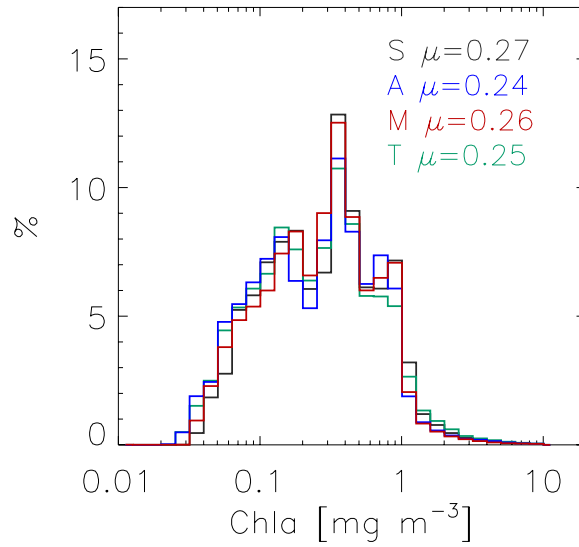
Fig. 2. Frequency distribution of multi-annual Chl-a (with histogram bins of 0.1 in logarithm of Chl-a). The geometric average \mu of the distribution is given for each sensor product, indicated by its reference letter ( S for SeaWiFS, A for MODIS Aqua, M for MERIS, and T for MODIS Terra).
