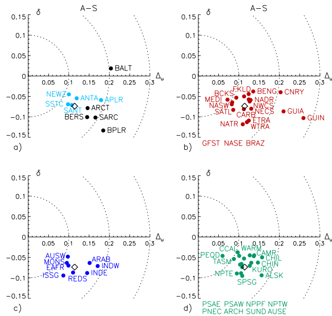
Fig. 6. Target diagram for the pair A-S (MODIS Aqua versus SeaWiFS), plotting bias \delta versus unbiased RMS difference \Delta_u , computed for each province and averaged over 2003-2007. The provinces are display per basin: (a) Arctic and Southern Ocean provinces (black and light blue, respectively), (b) Atlantic Ocean, (c) Indian Ocean, and (d) Pacific Ocean. The dashed circles are isolines of equal RMS difference \Delta . The global averaged statistics are indicated by a black diamond. To avoid cluttering, some province acronyms (close to the global average) are listed below the diagram.
