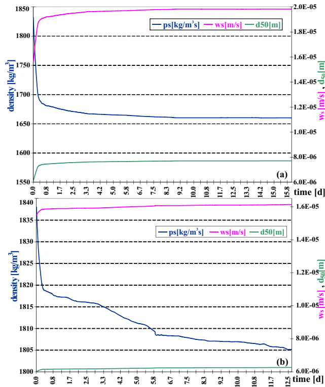
Fig. 7. Variation of sediment characteristics with time from introduction to the flow (blue line indicates particle density, magenta line denotes settling velocity and green line represents sediment characteristic diameter).
