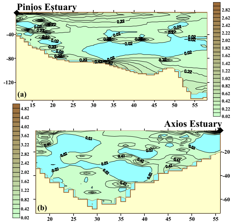
Fig. 10. Concentrations of suspended sediments, in mg/l, in cross-sections \alpha-\alpha (a) and \beta-\beta (b) for winter conditions from the S1A2 run. The vertical axis is the water depth (m) and the horizontal denotes the horizontal position in number of discretization steps ( dx=dy=1/60^\circ ).
