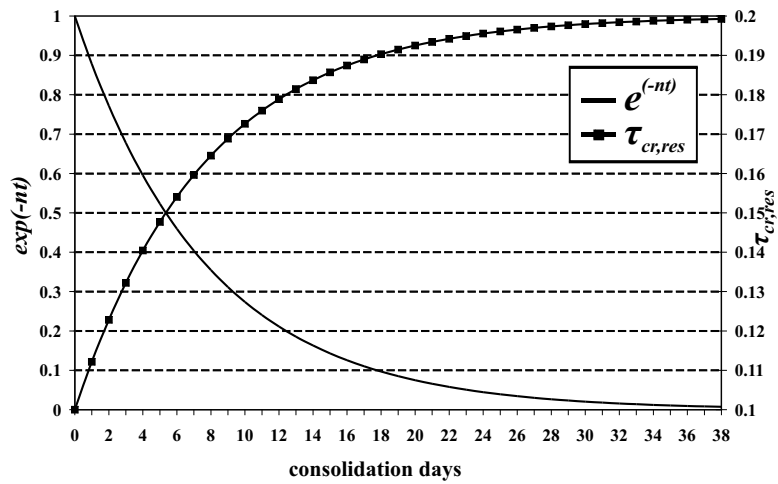
Fig. 1. Evolution of the exponential term in Eq. (19) (left axis) and the critical shear stress for resuspension of deposited sediments (right axis) with depositional time.
